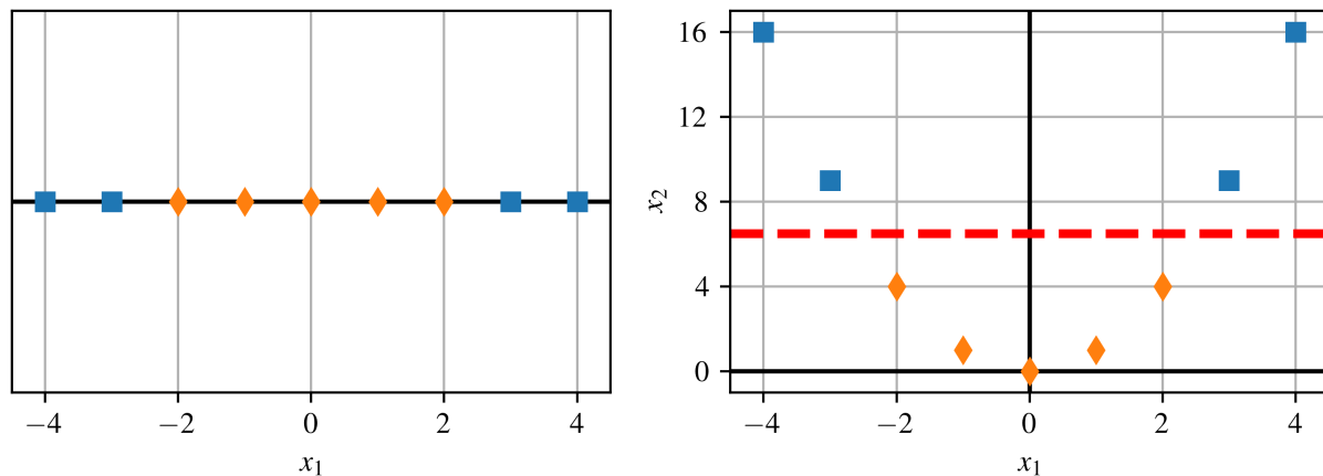
Figure 8.8: Illustration of SVM in higher dimensions
