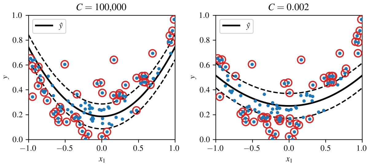
Figure 8.12: SVM regression with a 2 nd -degree polynomial kernel, showcasing different regularization levels.
