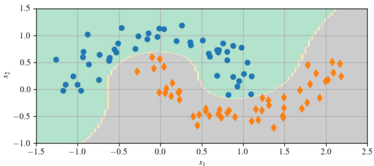
Figure 8.9: Demonstration of a SVM classifier with polynomial features.
