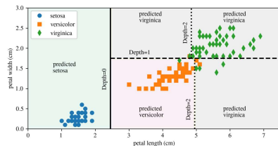
Decision tree decision boundaries.
