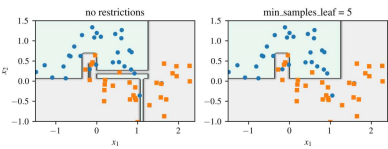
Regularization using min_samples_leaf .
