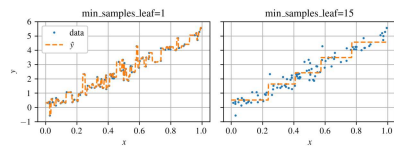
Effect of min_samples_leaf on regression trees.
