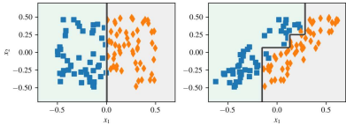
Sensitivity to feature rotation.
