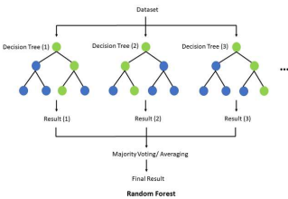
Random forest with majority voting.
