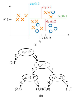
Basic concept of a decision tree.
