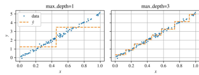
Regression trees with different depths.
