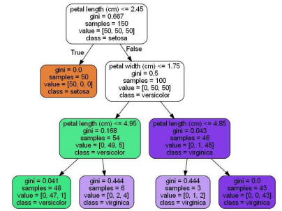
Decision tree trained on the Iris dataset.
