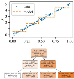
Decision Tree regression model and tree.
