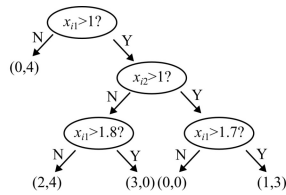
Basic concept of a decision tree.
