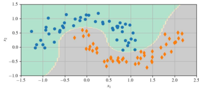
SVM classifier with polynomial features.
