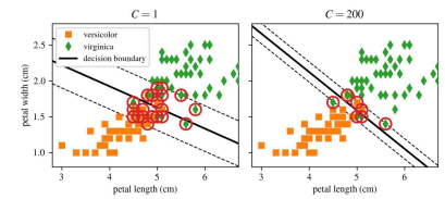
Effect of the C hyperparameter.
