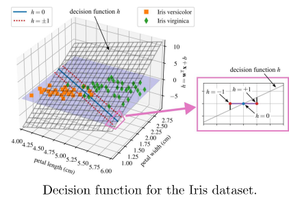
Decision function for the Iris dataset.
