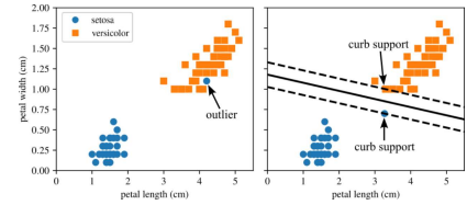
Hard margin sensitivity to outliers.
