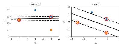
Effect of feature scaling.
