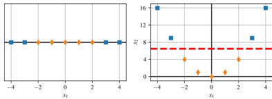
SVM in higher dimensions.
