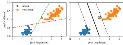
Large margin classification.
