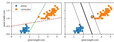
The boundary is shaped by the support vectors.
