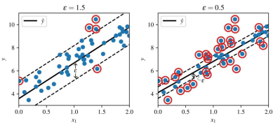
Linear SVR with different \epsilon values.
