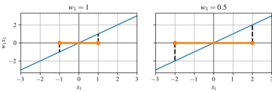
Smaller weights produce a larger margin.
