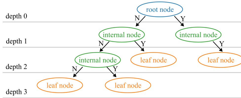
Figure 6.4: Illustration of the CART algorithm process.
