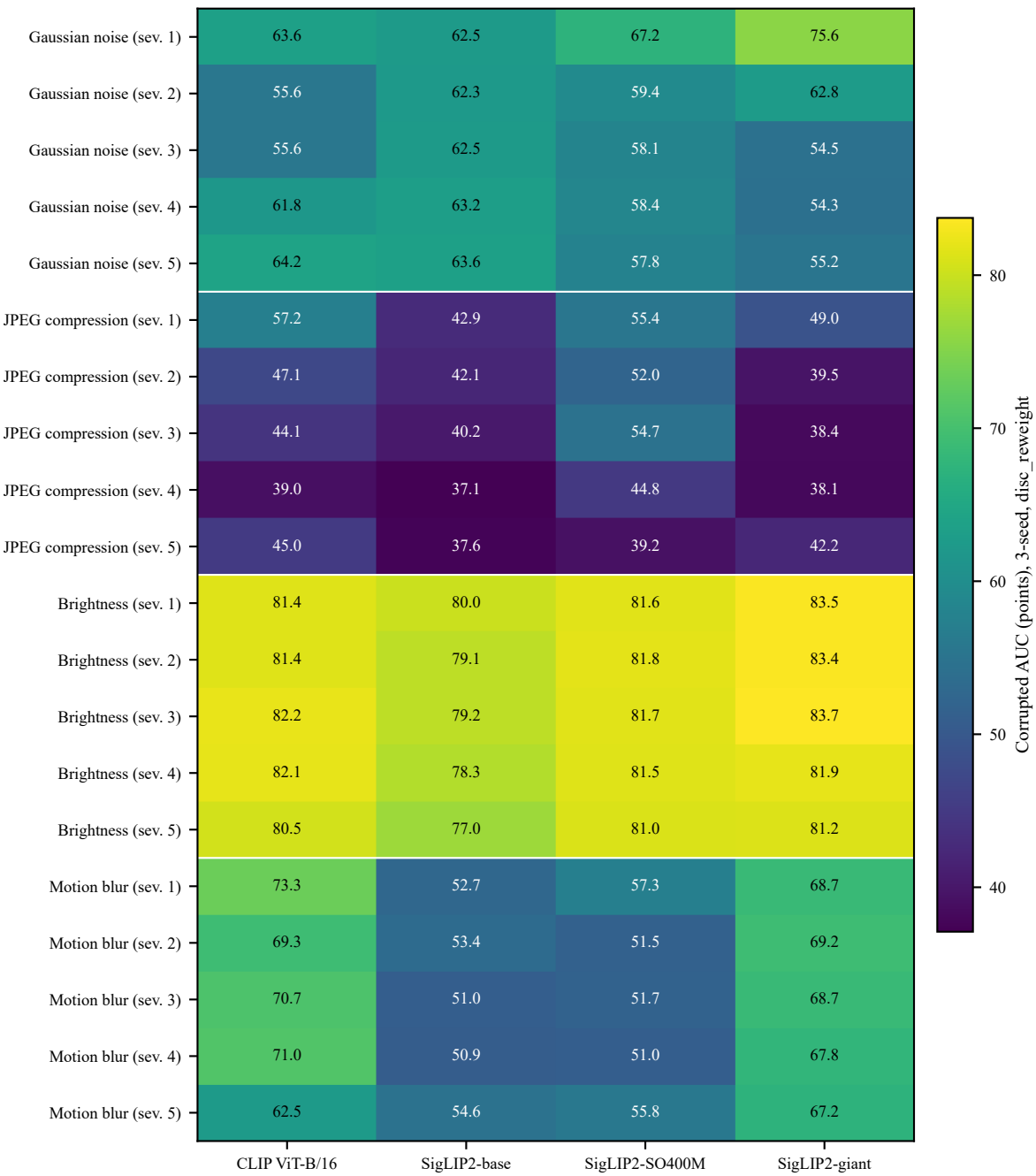
disc_reweight corrupted AUC on UCF-Crime-C (3-seed mean, points)
