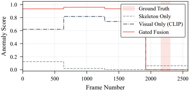
RoadAccidents127 (RoadAccidents)
