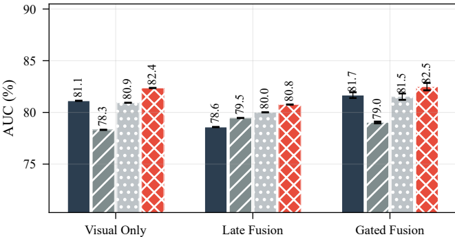
UCF-Crime
