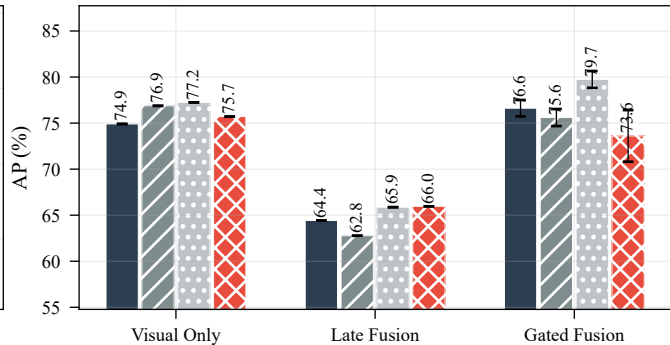
XD-Violence
