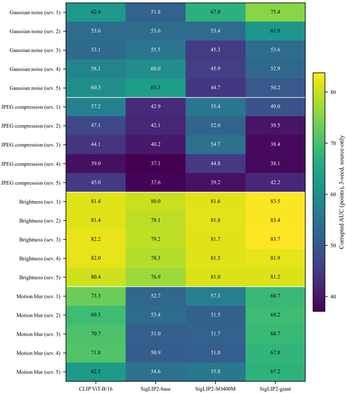
Source-only corrupted AUC on UCF-Crime-C (3-seed mean, points; no adaptation)
