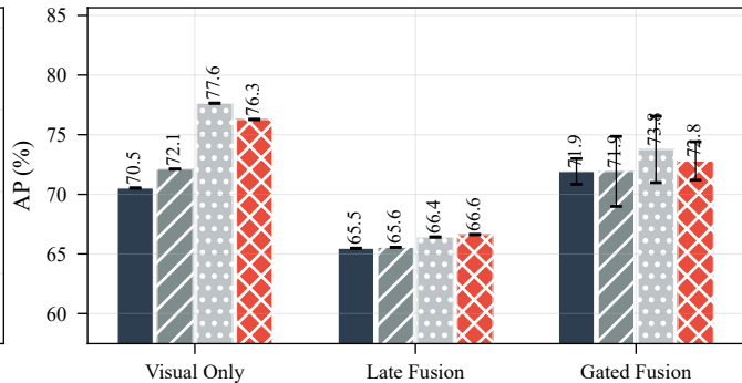
XD-Violence
