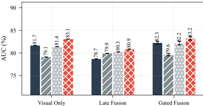
UCF-Crime
