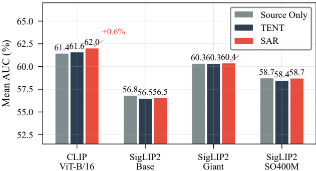
TTA Methods Across Backbones (20 Corruptions)
