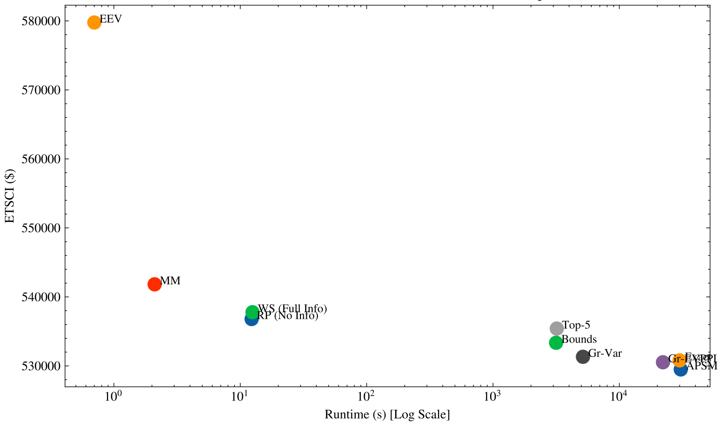
Pareto Trade-off: Runtime vs. ETSCI (15x15 Setup)
