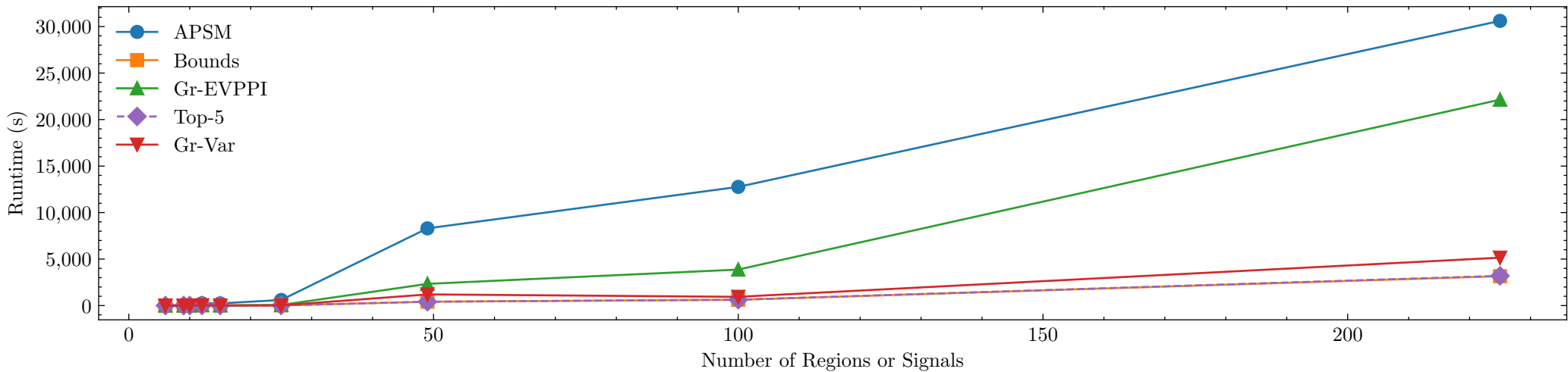
Algorithm Scalability: Runtime vs. Network Size
