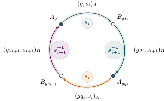
Figure 1: A face from Lemma 3.2. Each arrow is labeled by its dart and, in bold, its group multiplier. Adapted from [11].
