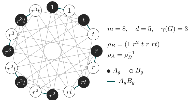
Figure 3: The odd-degree dihedral group example H(D_4, \{1, r^2, t, r, rt\}) .
