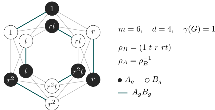
Figure 2: The even-degree dihedral group example H(D_3, \{1, t, r, rt\}) .
