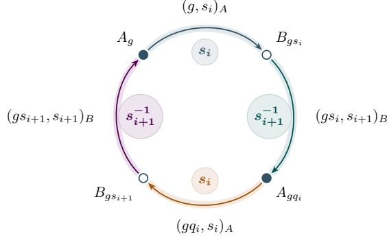
Figure 1: A face of Lemma 3.2. Each arrow is labeled by its dart and its group multiplier [11].
