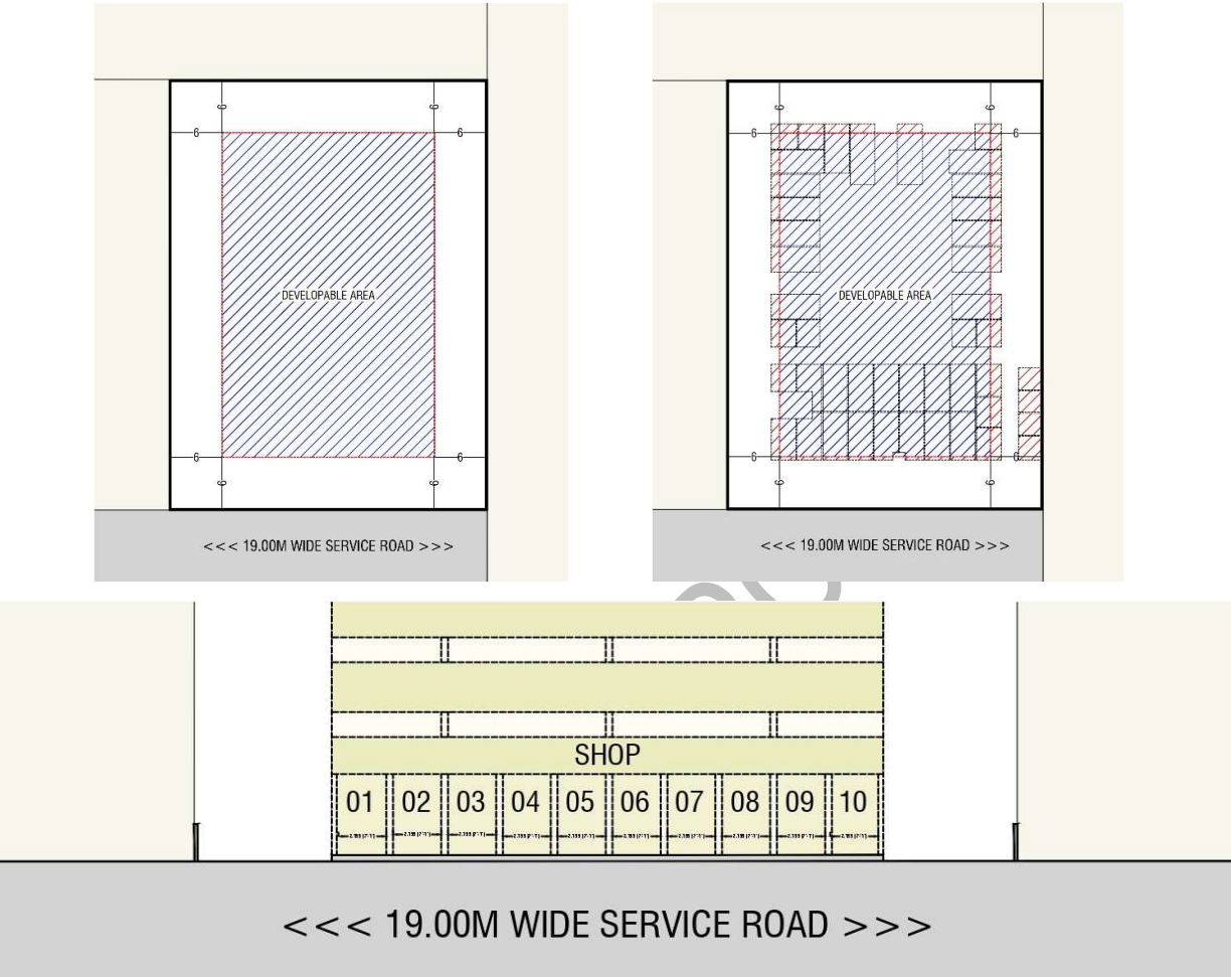
Schematic section for Proposed Commercial Building
