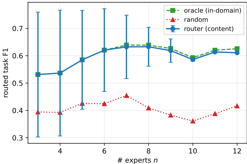
(A1) Routing quality vs expert count
