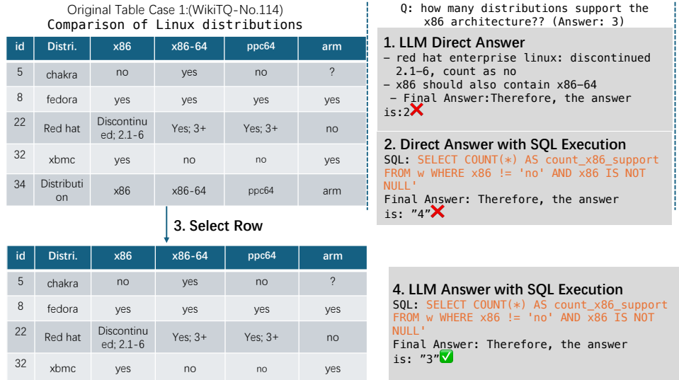
Fig. 8: Failure modes in semantic and categorical TQA. This case asks, "how many distributions support the x86 architecture?" (Correct Answer: 3). The LLM's direct answer incorrectly yields "2" by misinterpreting the context of "discontinued" and confusing "x86" with "x86-64", showcasing its shortage in semantic understanding with irrelevant context. Direct SQL-based answer incorrectly counts "4" due to its inability to filter out last row as header, again demonstrating the limited fault tolerance of symbolic methods for dirty tables.
