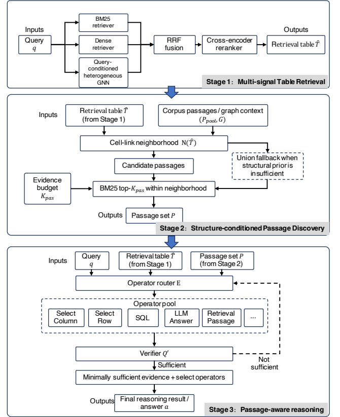
Fig. 4: Overview of SPARQ+. Stage 1 retrieves a table \hat{T} by fusing lexical, semantic, and structural retrieval signals. Stage 2 discovers passages P from the cell-link neighborhood of \hat{T} under evidence budget K_{\text{pas}} . Stage 3 performs passage-aware routing and verification over (q, \hat{T}, P) to produce the answer.
