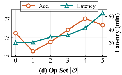
Fig. 10: Additional Hyperparameter Analysis of operator set expansion for SPARQ 4B on WikiTQ dataset.
