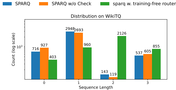
Fig. 17: Distribution of |S| on WikiTQ by SPARQ 4B .
