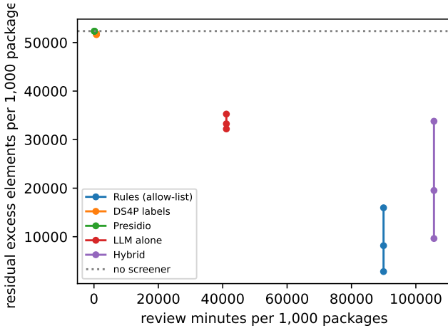
Fig. 2. Residual excess against review minutes per 1,000 packages at one minute per flag, across reviewer agreement levels.
