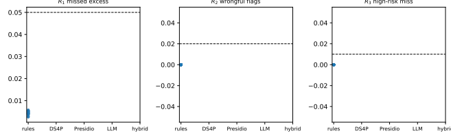
Fig. 1. Empirical test risks at the certified threshold across 20 splits (dots) against the targets (dashed). Screeners without a dot abstained in every split.
