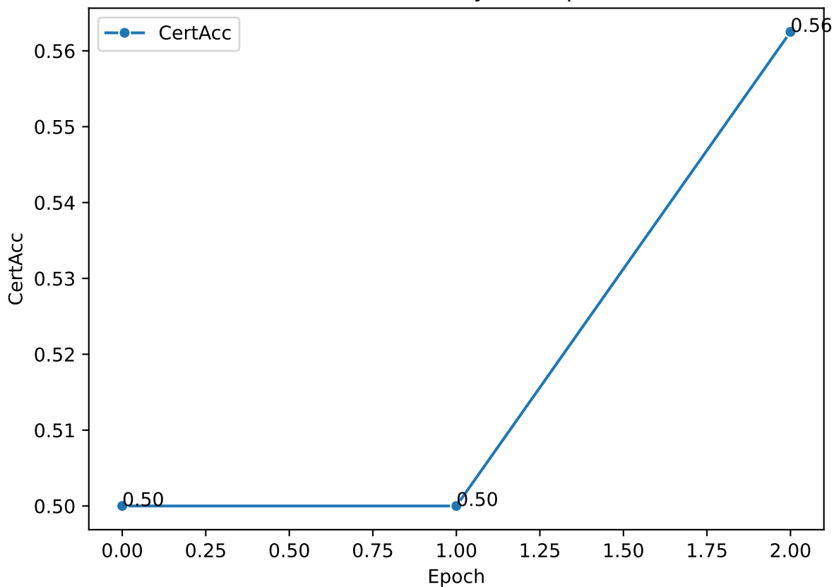
Certified Accuracy over Epochs
