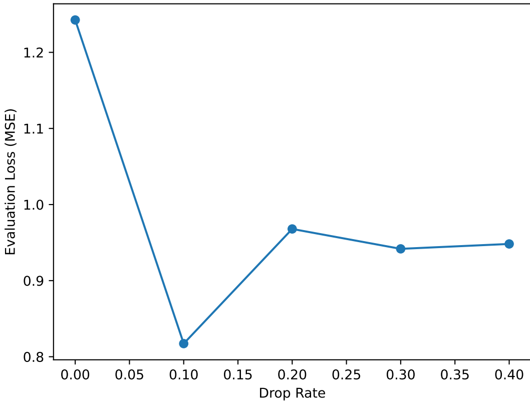
OOD Evaluation: Loss vs Token Drop Rate
