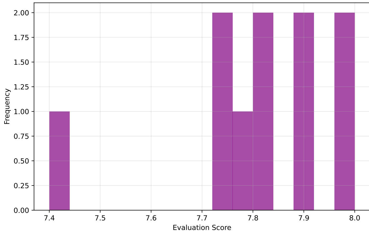
Score Distribution
