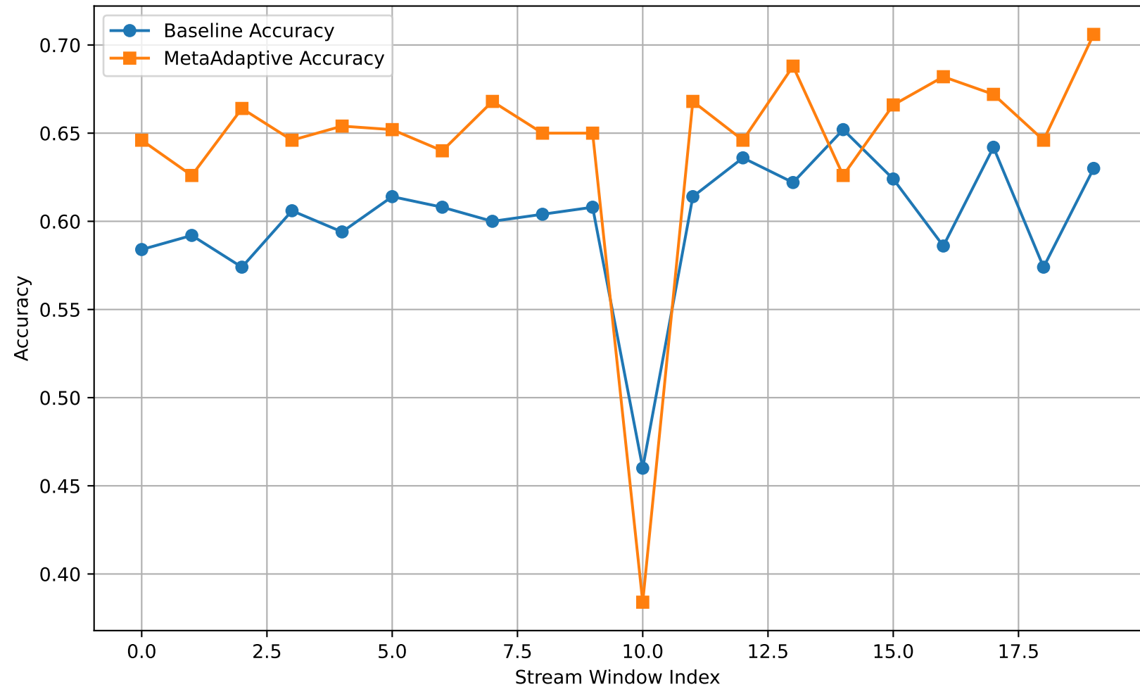
Performance Comparison with Concept Drift
