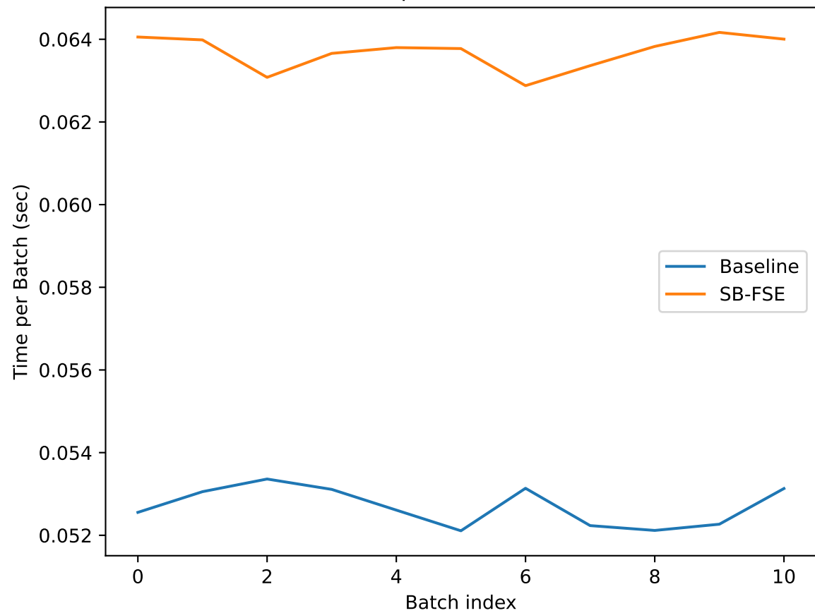
Computational Cost
