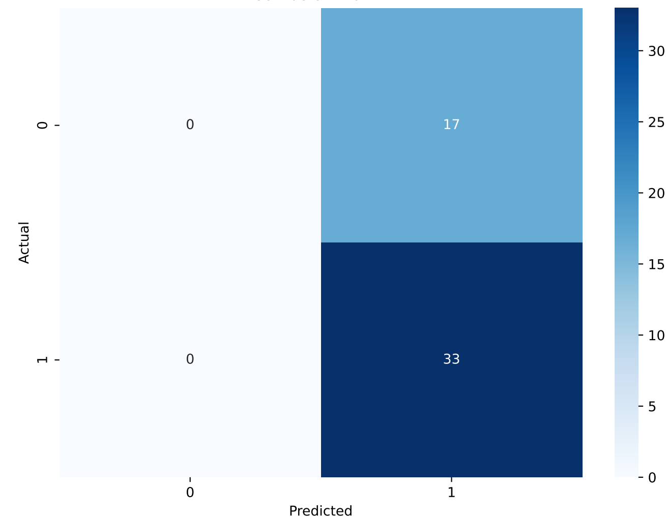
Confusion Matrix
