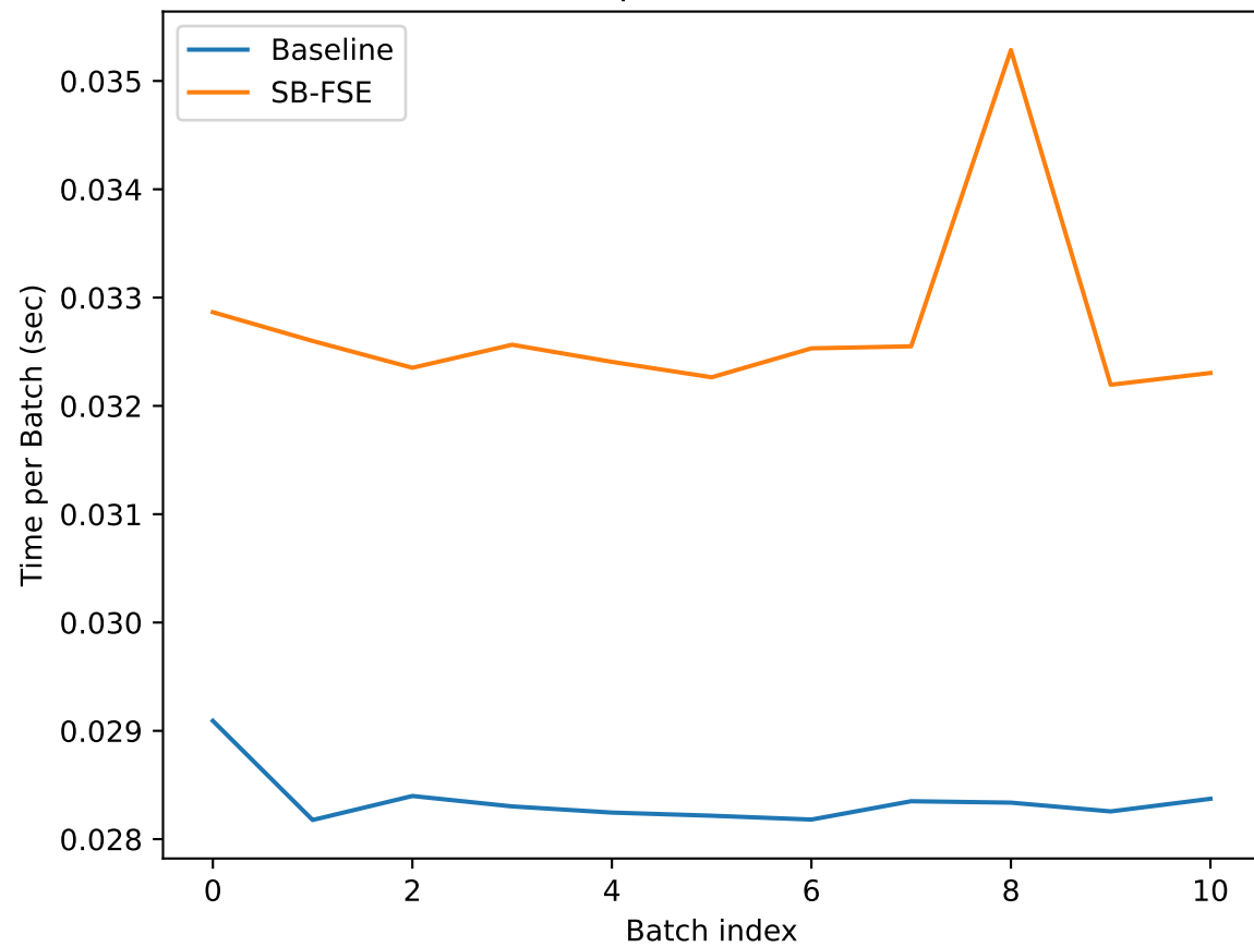
Computational Cost
