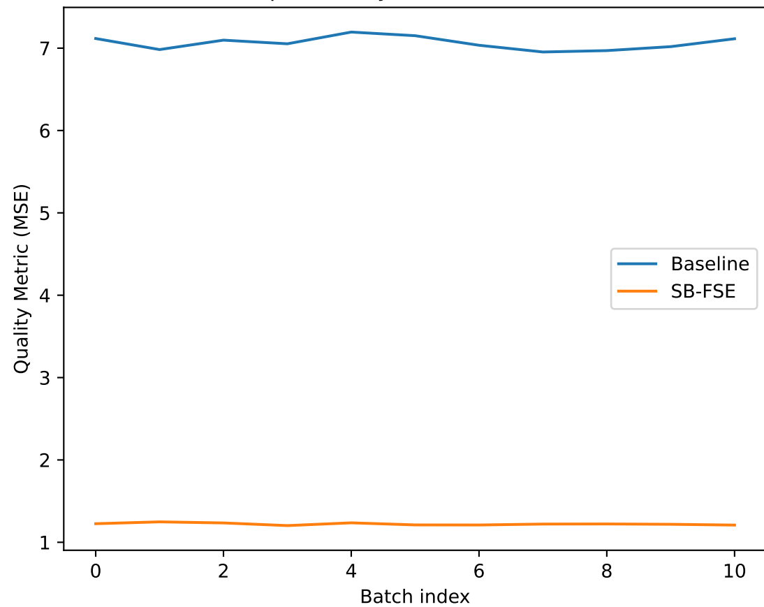
Sample Quality under Added Noise
