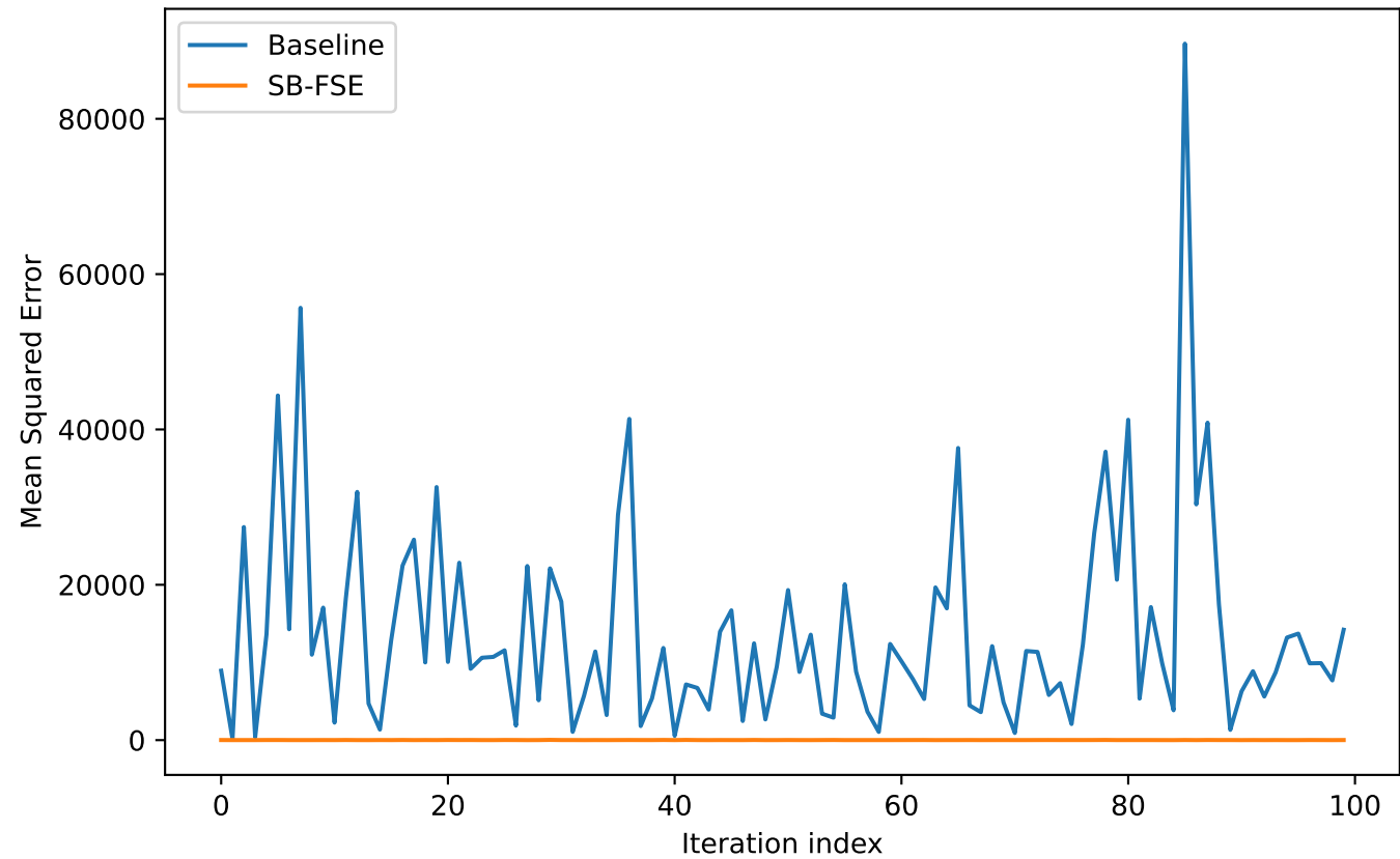
Convergence Comparison: Baseline vs SB-FSE
