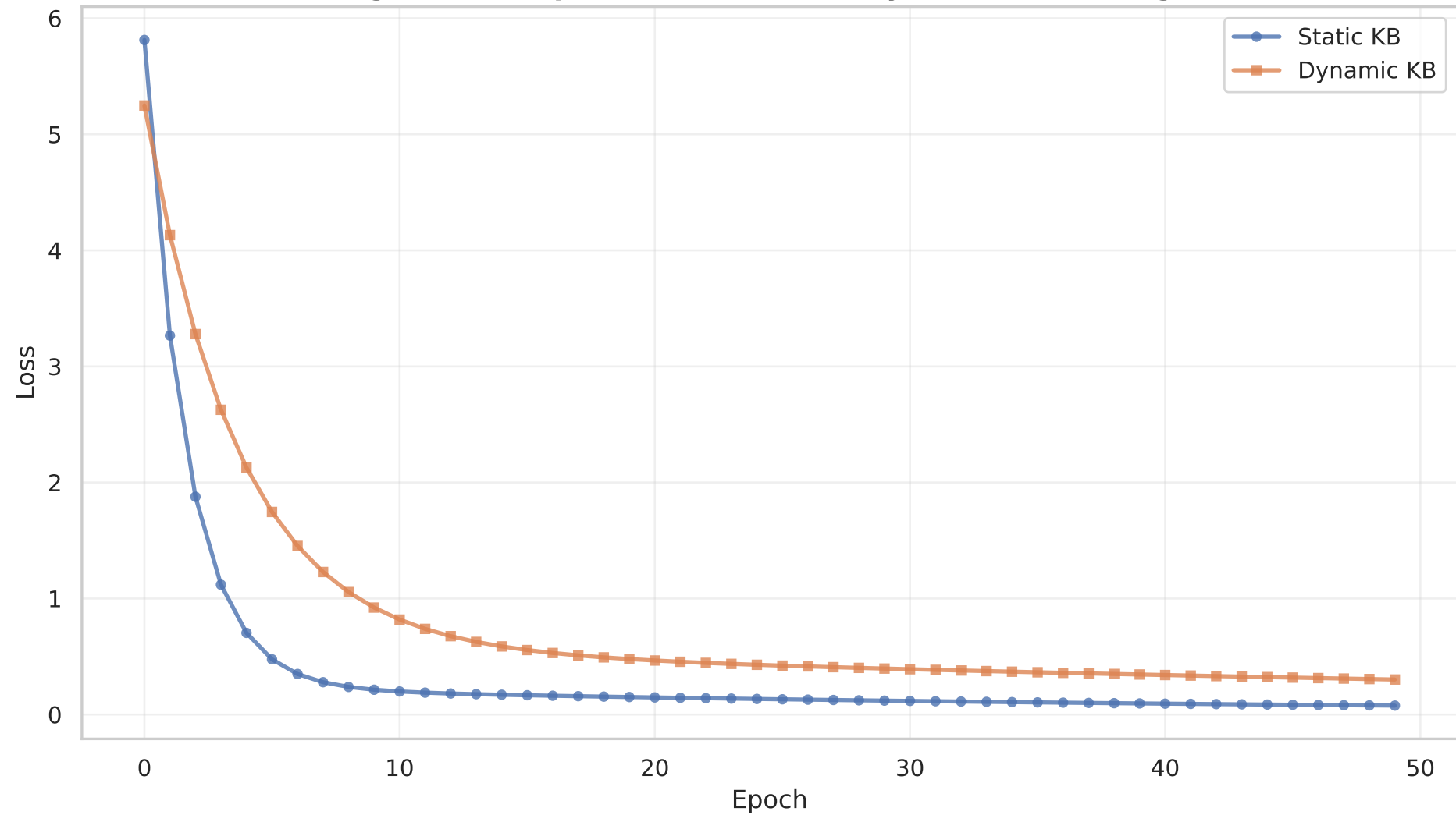
Training Loss Comparison: Static vs. Dynamic Knowledge Base
