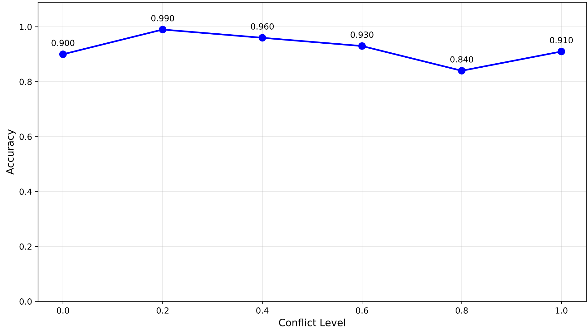
Robustness to Conflicting Modalities
