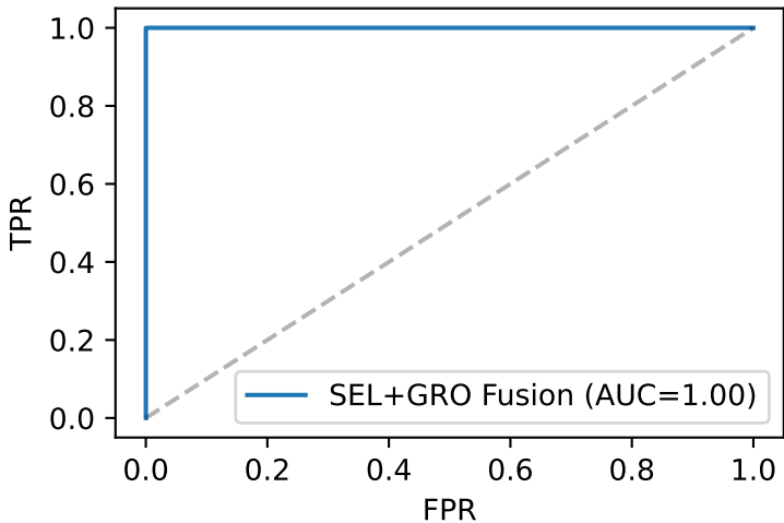
ROC (black-box)
