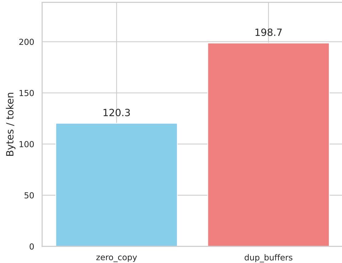
KV-Cache Memory Traffic
