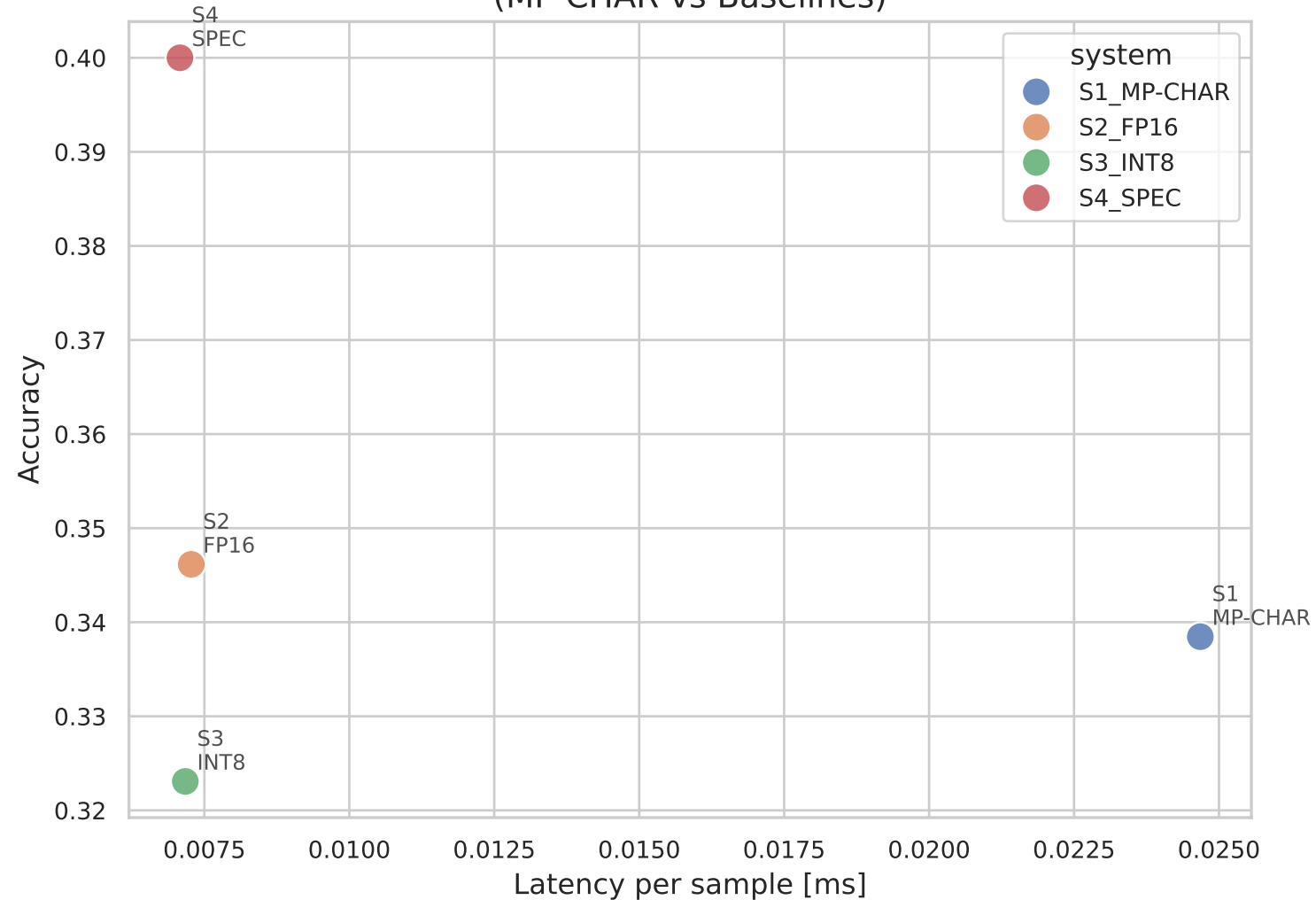
Quality-Latency Pareto Frontier (MP-CHAR vs Baselines)
