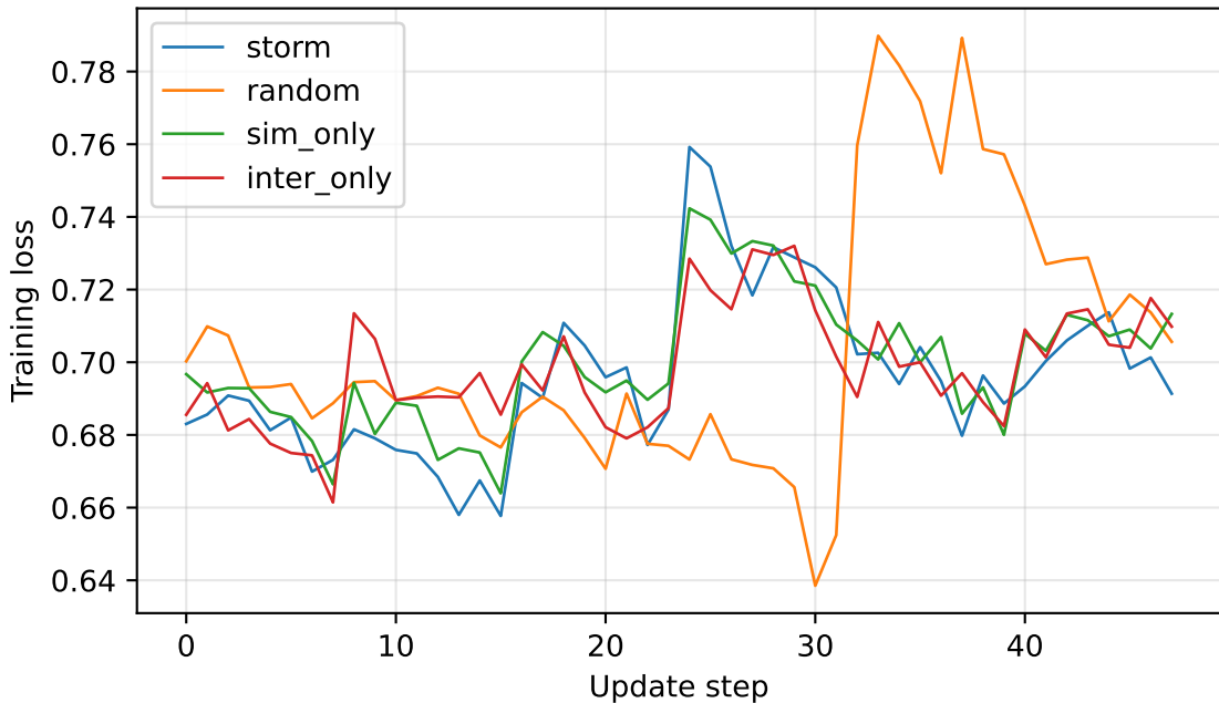
Training loss over time
