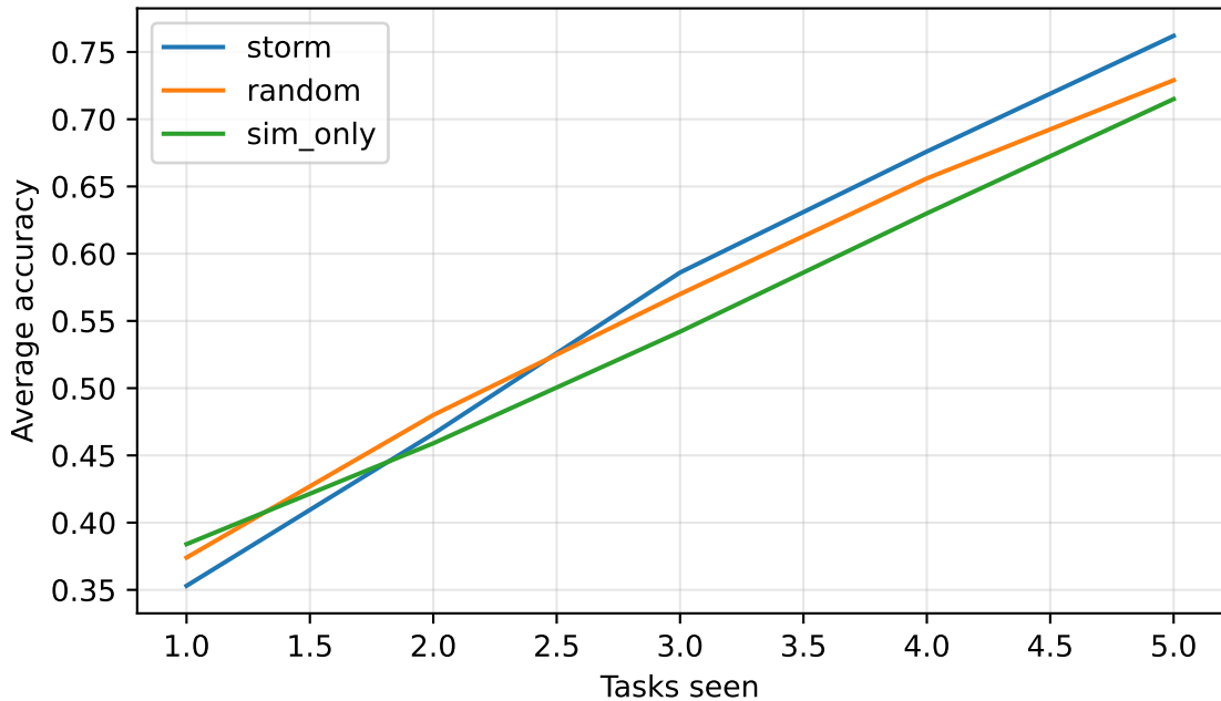
Average accuracy over sequence
