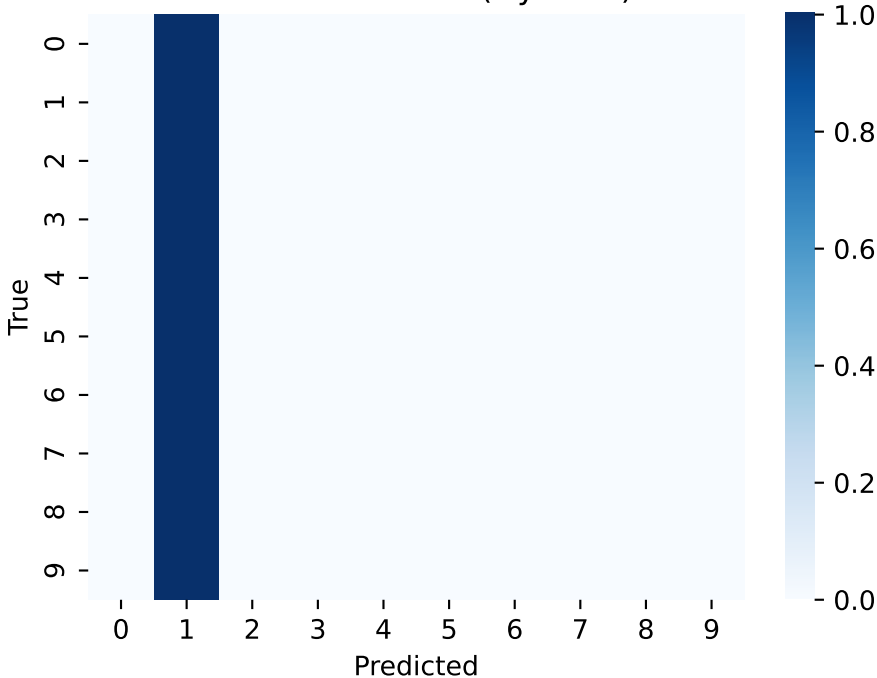
Confusion Matrix (DyCLOS)
