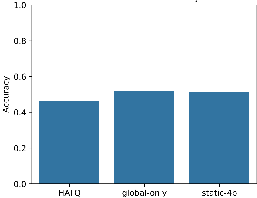
Classification accuracy
