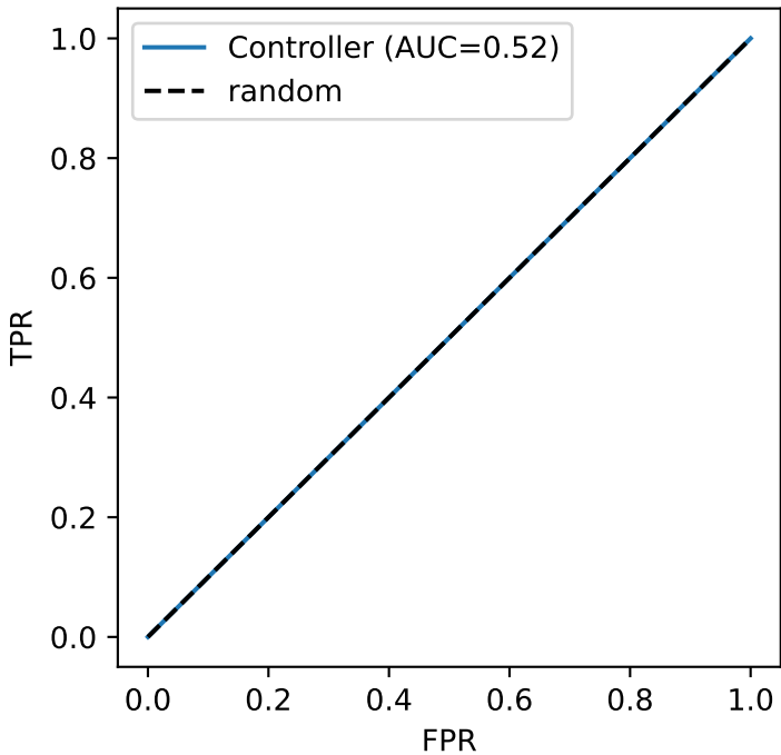
Controller ROC
