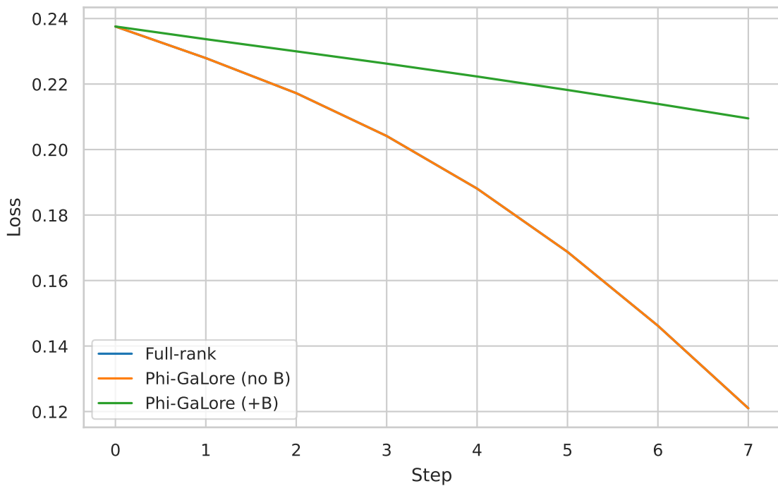
Training Loss (Navier-Stokes toy)
