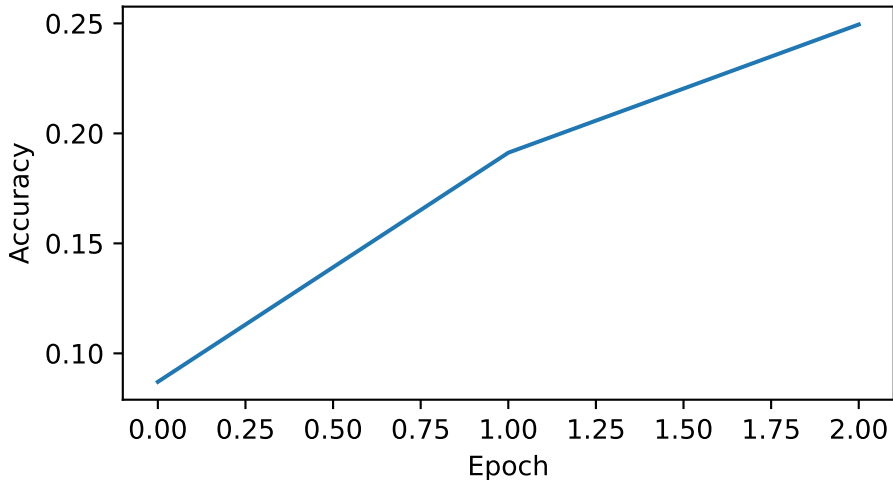
Validation Accuracy
