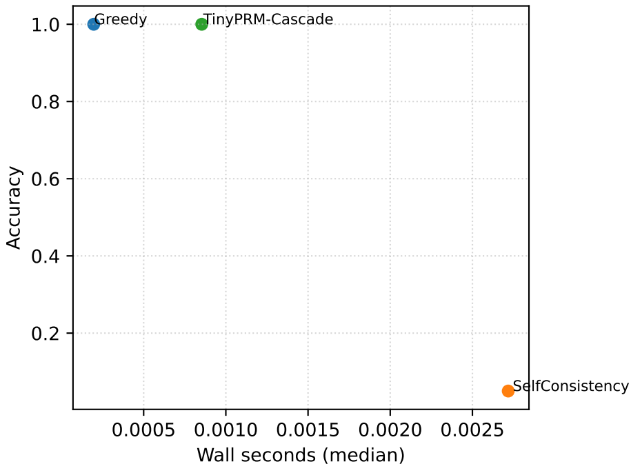
Accuracy vs Compute Pareto
