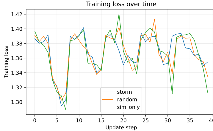
Figure 6: Training loss over time for the NLP proxy.
