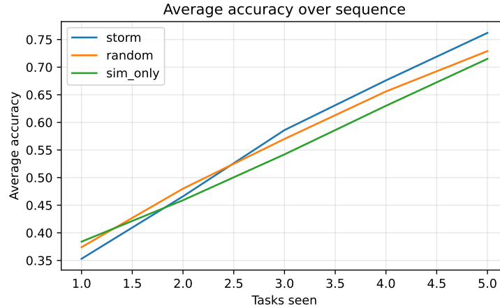
Figure 5: Accuracy over time for the NLP proxy (synthetic bag-of-words).
