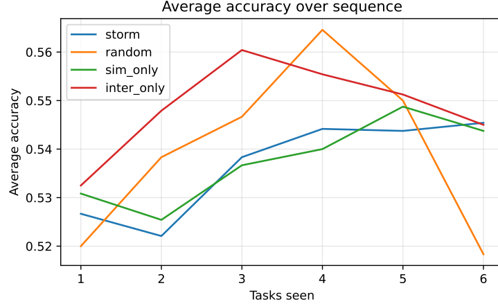
Figure 1: Accuracy over time for the synthetic experiment, STORM vs baselines.
