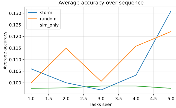
Figure 3: Accuracy over time for the vision proxy (split CIFAR-10).
