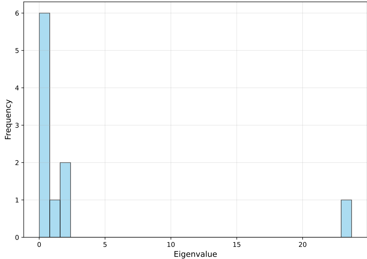
Eigenvalue Distribution for Block 2
