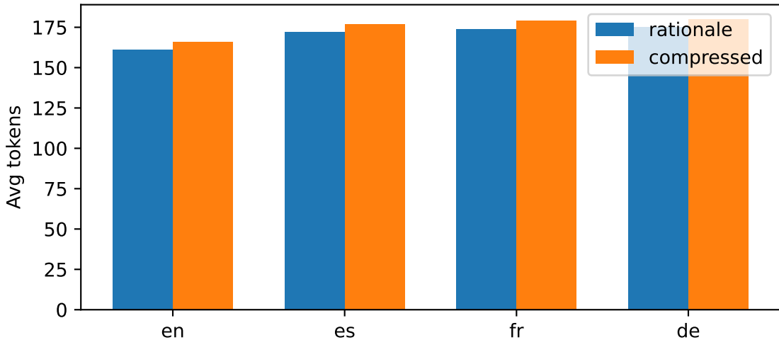
Output length by language (Exp3)
