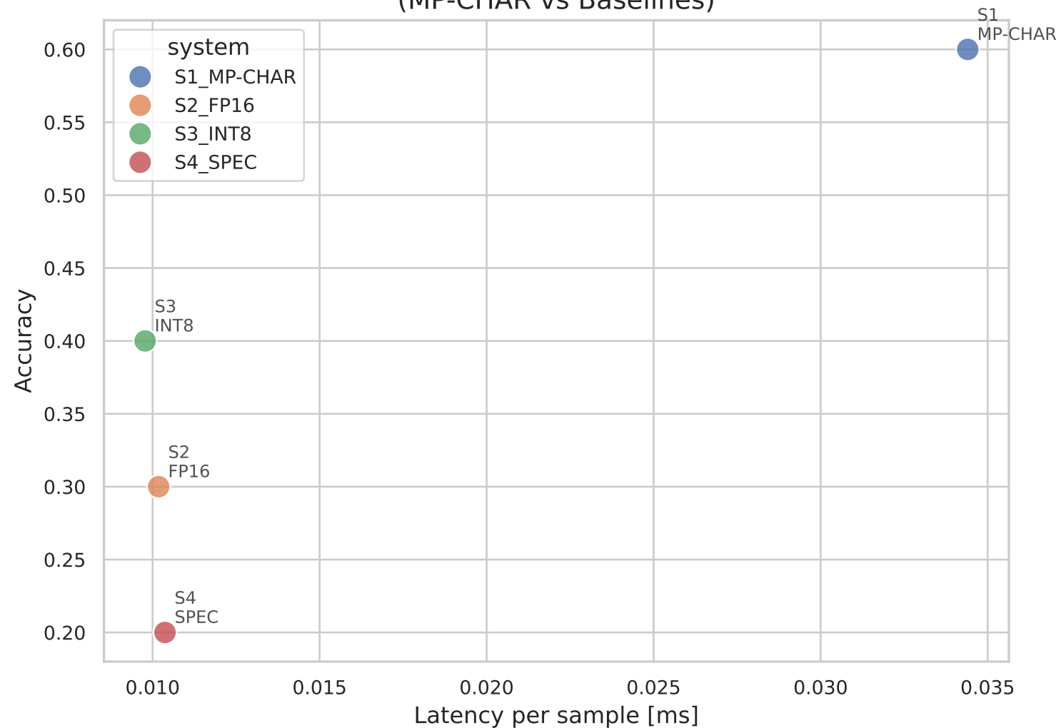
Quality-Latency Pareto Frontier (MP-CHAR vs Baselines)
