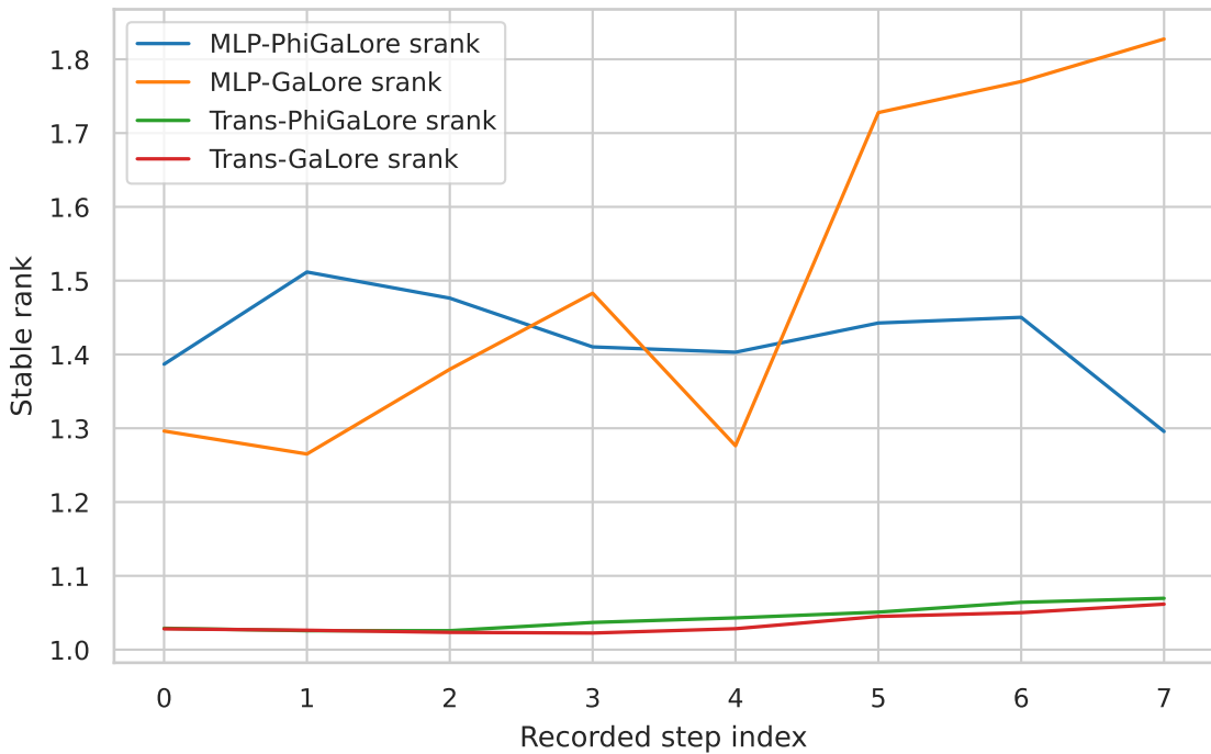
Gradient Stable Rank
