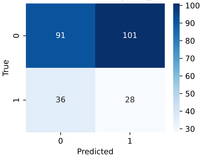
Confusion matrix (HATQ)
