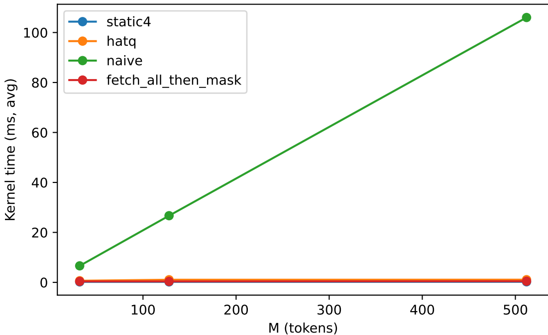
Systems micro-bench: mixA
