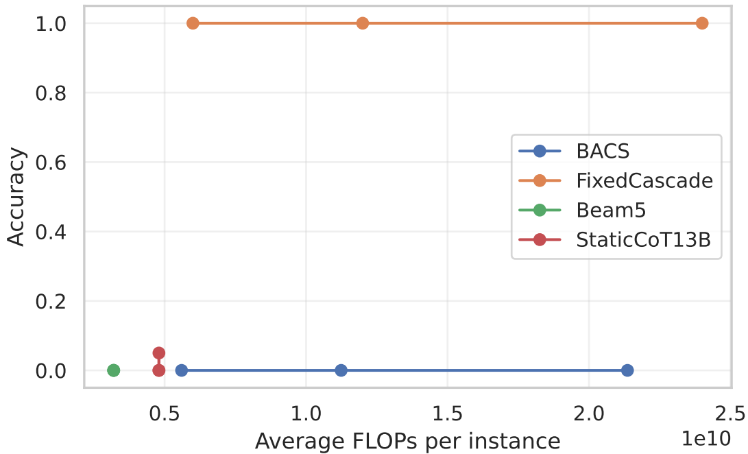
Accuracy vs Compute (BACS vs baselines)
