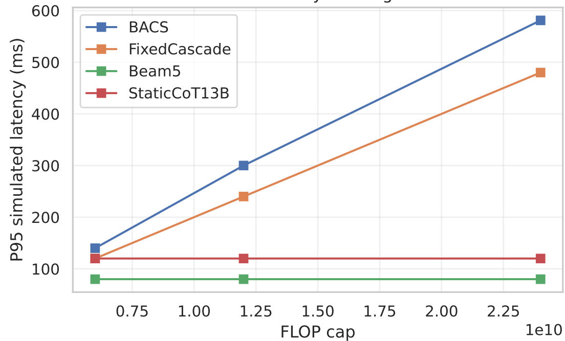
P95 latency vs budget
