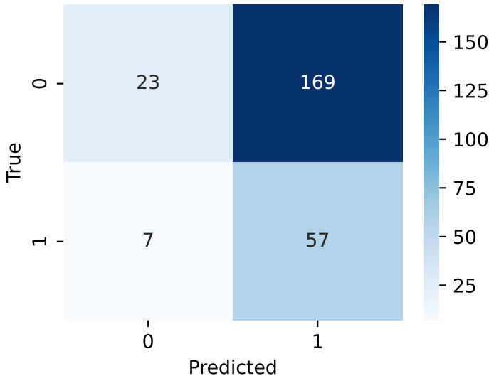
Confusion matrix (HATQ)
